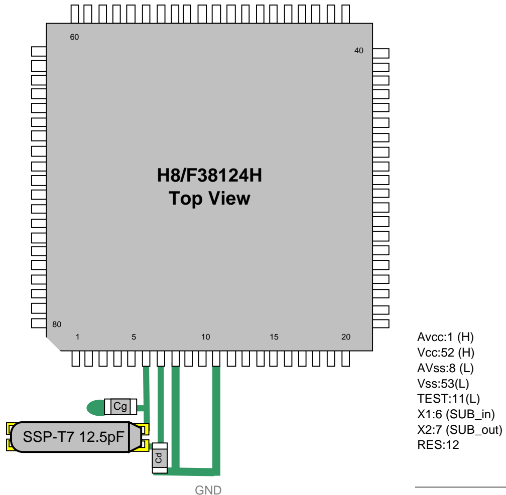
Figure 1 Referencial components layout
