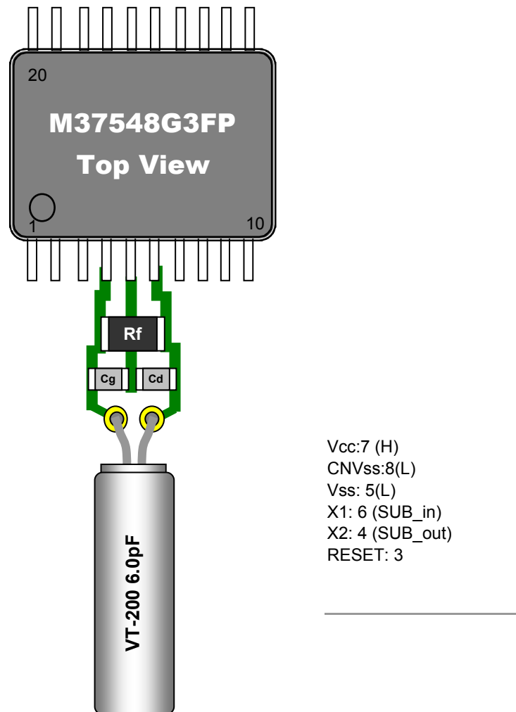
Figure 1 Referential components layout
